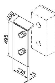
PZPS 140 02 Front protection plate for rubber buffer PGF 140
