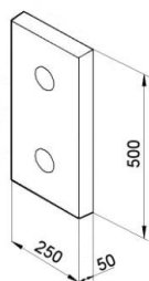
PEHD 500x250x50 Polyethylene buffer
