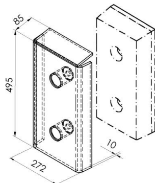
PZPS 90 07 Front protection plate for rubber buffer PGF 90
