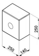
PBGP 250x250x140 Rubber buffer
