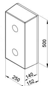
PGF 140 Rubber buffer on hot-dip galvanized plate
