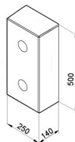
PBGP 500x250x140 Rubber buffer
