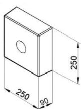
PBGP 250x250x90 Rubber buffer
