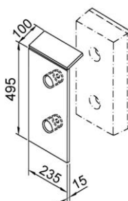
PZPS 90 02 Front protection plate for rubber buffer PGF 90
