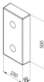
PBGP 500x250x90 Rubber buffer
