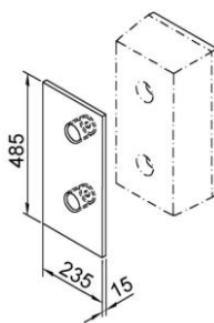
PZPS 140 01 Front protection plate for rubber buffer PGF 140
