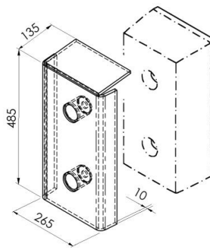
PZPS 140 07 Front protection plate for rubber buffer PGF 140
