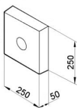
PEHD 250x250x50 Polyethylene buffer
