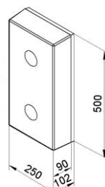
PGF 90 Rubber buffer on hot-dip galvanized plate
