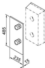
PZPS 90 06 Front protection plate for rubber buffer PGF 90
